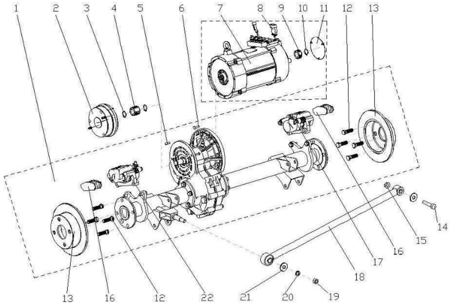
STANDARD REAR AXLE PARTS DIAGRAM CONTINUED
