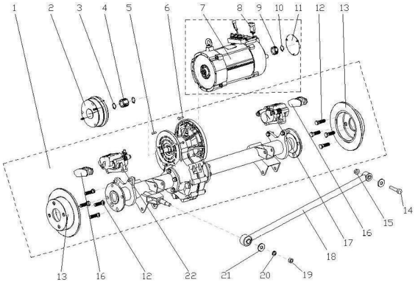
LIFTED REAR AXLE PARTS DIAGRAM
